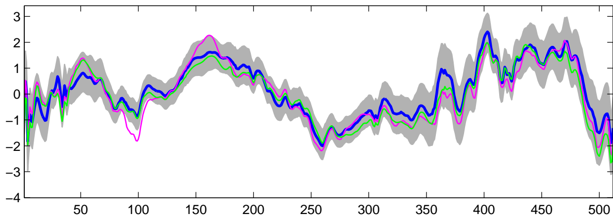
Estimated U_{11}(t) using R-WFMM: Normal data, run 8
