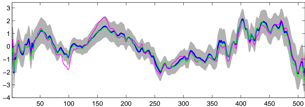
Estimated U_{11}(t) using G-WFMM: Normal data, run 8
