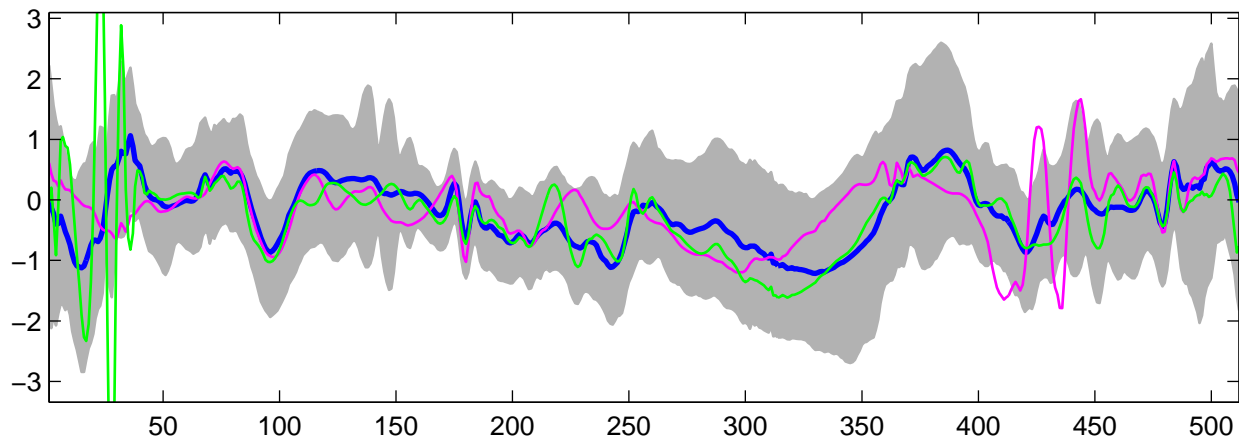
Estimated U_{11}(t) using G-WFMM: t_1 data, run 8
