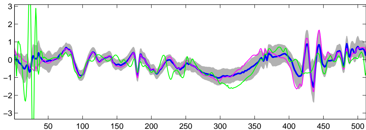
Estimated U_{11}(t) using R-WFMM: t_1 data, run 8
