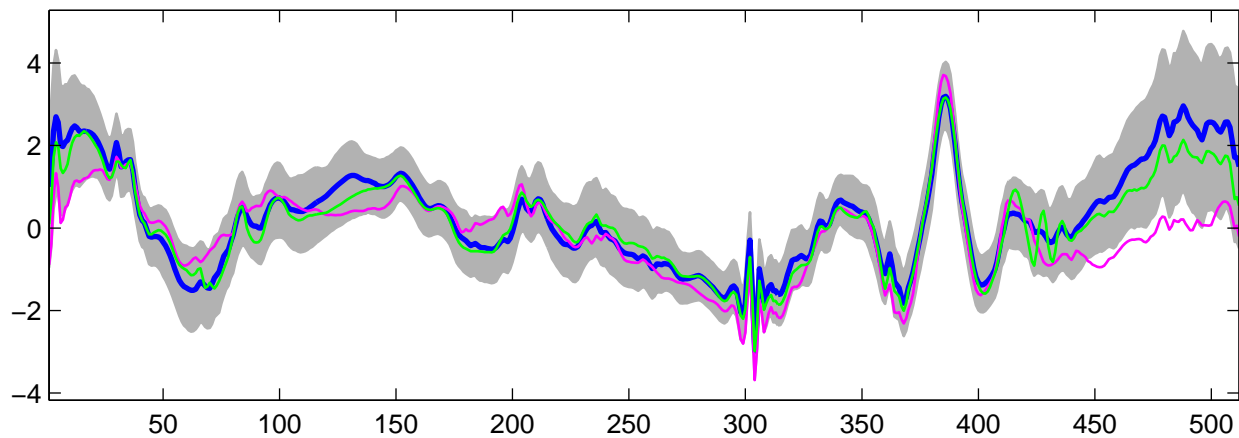
Estimated U_{11}(t) using G-WFMM: t_2 data, run 8
