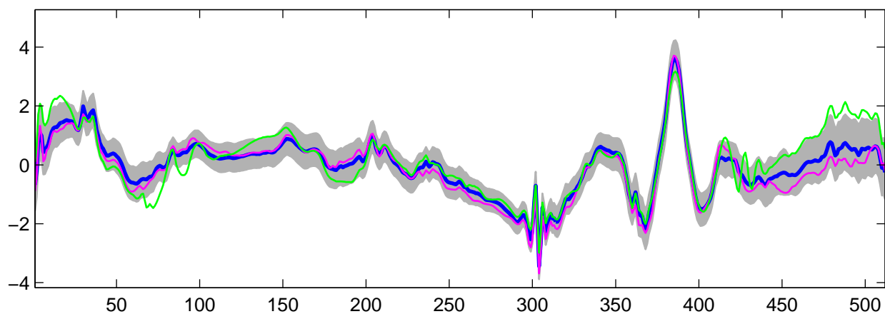
Estimated U_{11}(t) using R-WFMM: t_2 data, run 8
