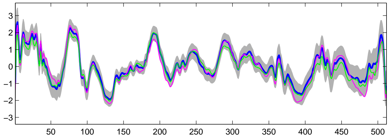
Estimated U_{11}(t) using R-WFMM: t_3 data, run 8
