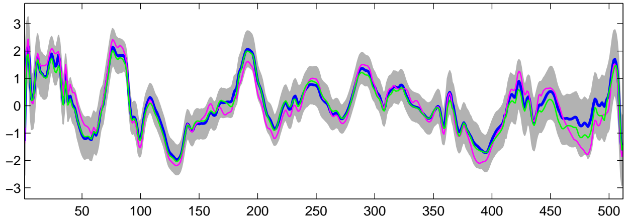
Estimated U_{11}(t) using G-WFMM: t_3 data, run 8
