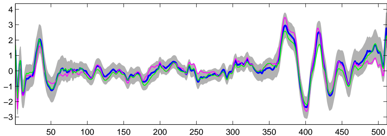
Estimated U_{12}(t) using R-WFMM: DE data, run 8
