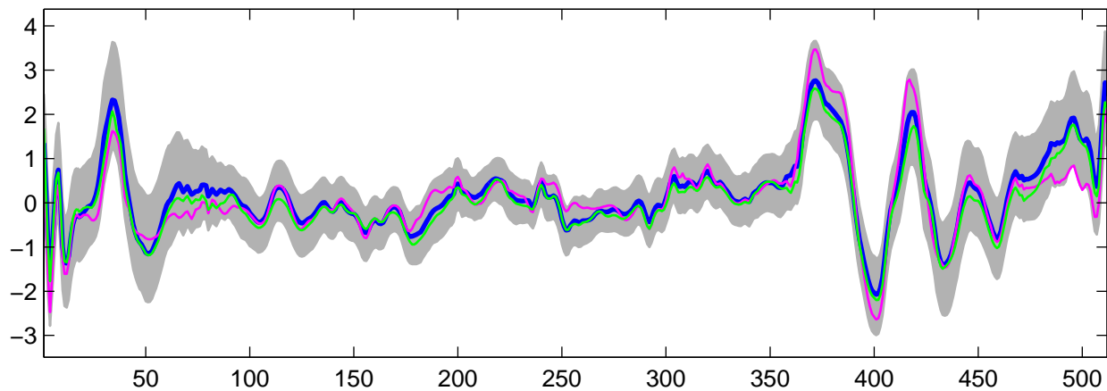
Estimated U_{12}(t) using G-WFMM: DE data, run 8
