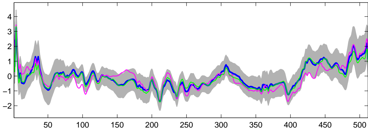
Estimated U_{12}(t) using G-WFMM: Normal data, run 8
