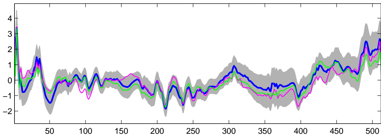
Estimated U_{12}(t) using R-WFMM: Normal data, run 8
