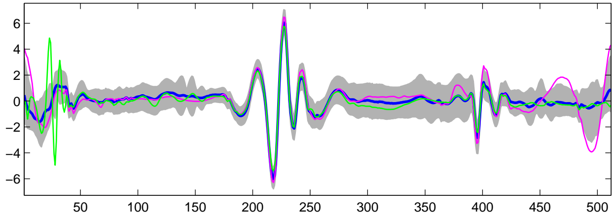
Estimated U_{12}(t) using G-WFMM: t_1 data, run 8
