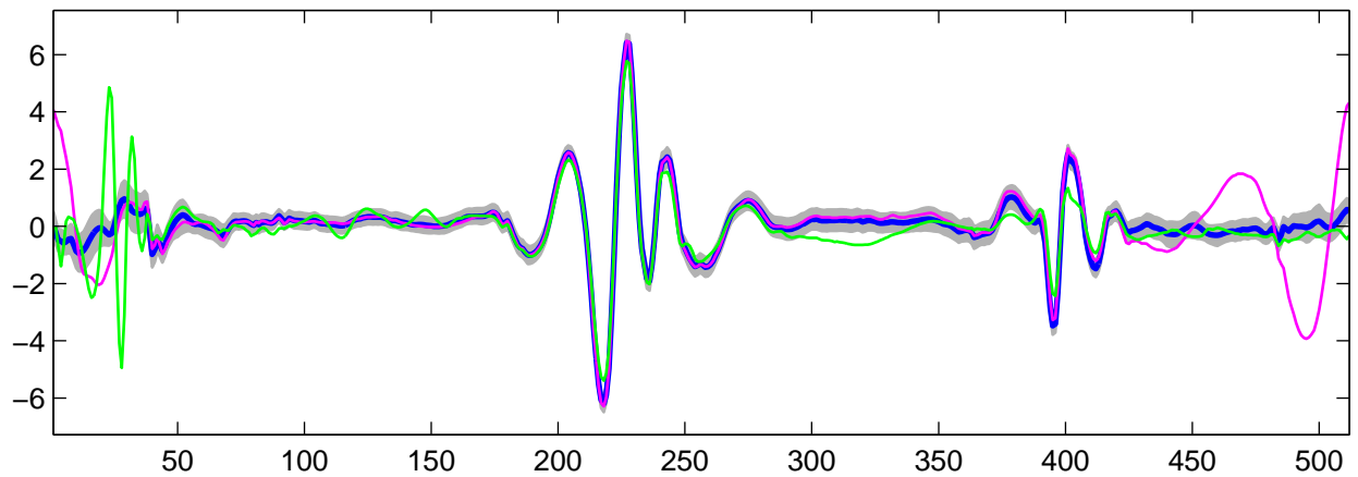
Estimated U_{12}(t) using R-WFMM: t_1 data, run 8
