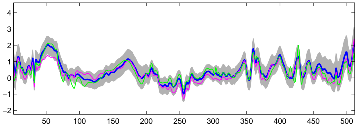
Estimated U_{12}(t) using R-WFMM: t_2 data, run 8
