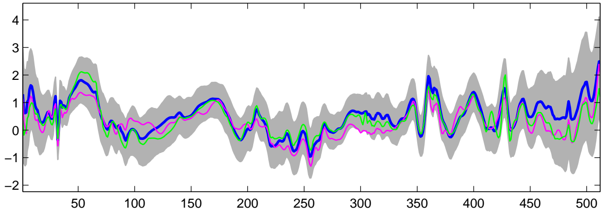
Estimated U_{12}(t) using G-WFMM: t_2 data, run 8
