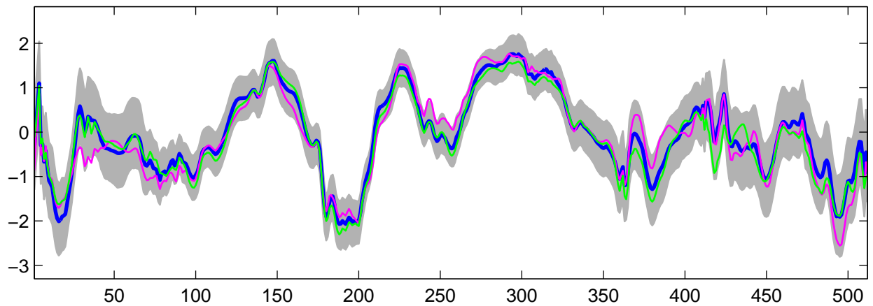
Estimated U_{13}(t) using R-WFMM: DE data, run 8
