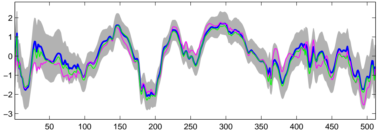
Estimated U_{13}(t) using G-WFMM: DE data, run 8
