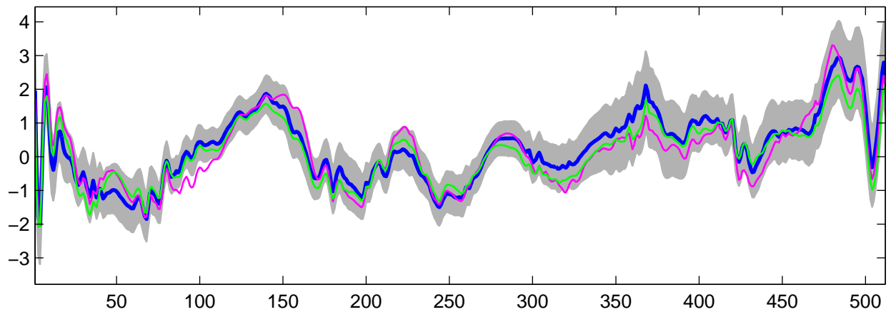
Estimated U_{13}(t) using R-WFMM: Normal data, run 8
