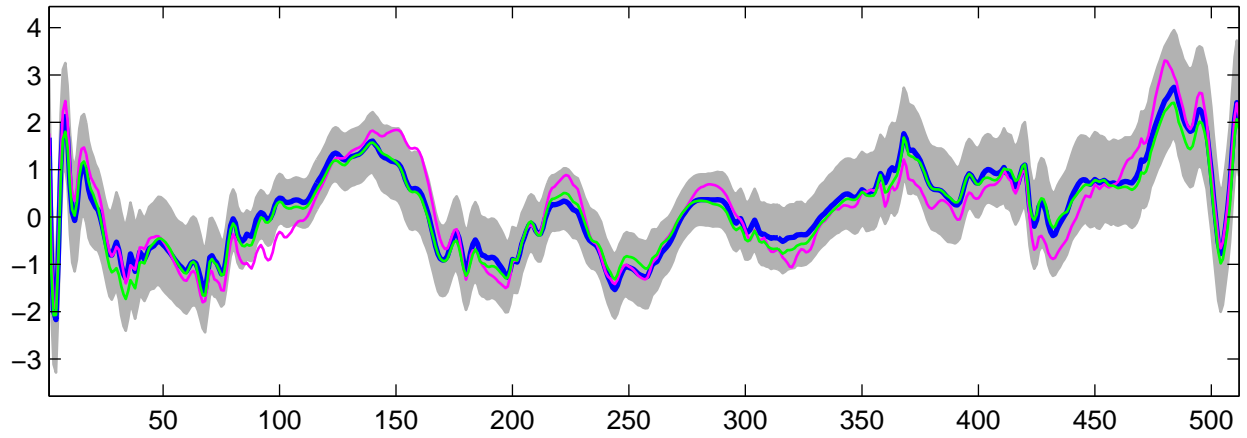
Estimated U_{13}(t) using G-WFMM: Normal data, run 8
