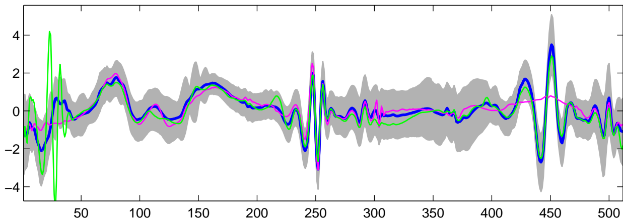
Estimated U_{13}(t) using G-WFMM: t_1 data, run 8
