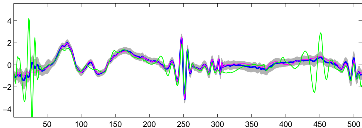
Estimated U_{13}(t) using R-WFMM: t_1 data, run 8
