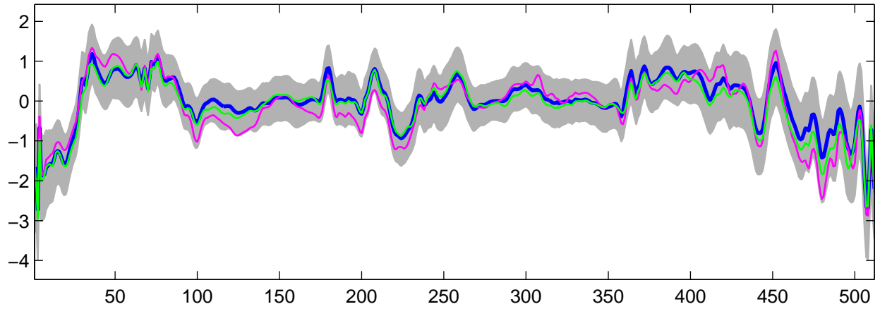
Estimated U_{13}(t) using G-WFMM: t_3 data, run 8
