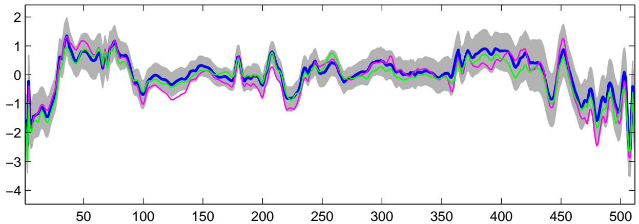
Estimated U_{13}(t) using R-WFMM: t_3 data, run 8
