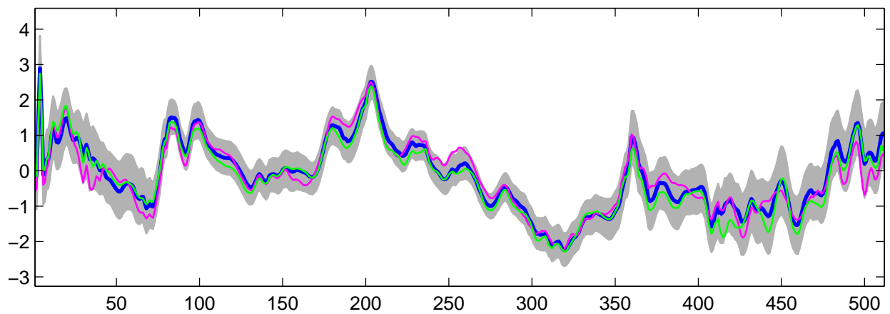
Estimated U_{14}(t) using R-WFMM: DE data, run 8
