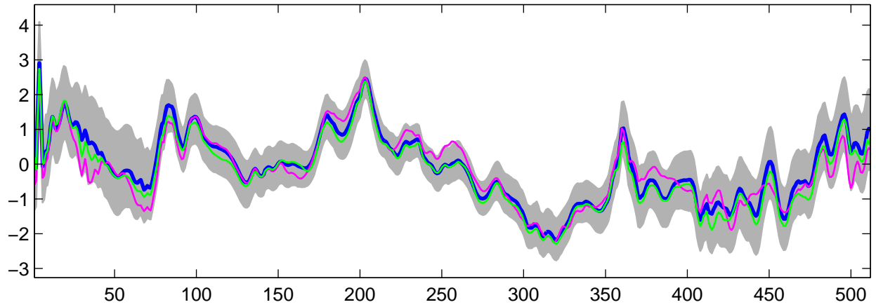
Estimated U_{14}(t) using G-WFMM: DE data, run 8
