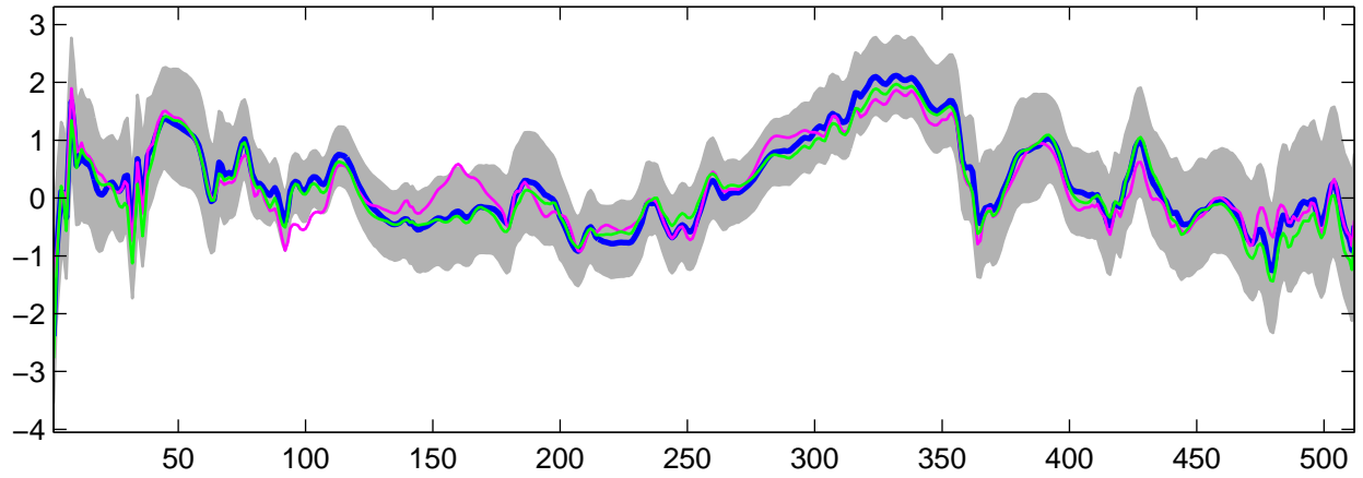
Estimated U_{14}(t) using G-WFMM: Normal data, run 8
