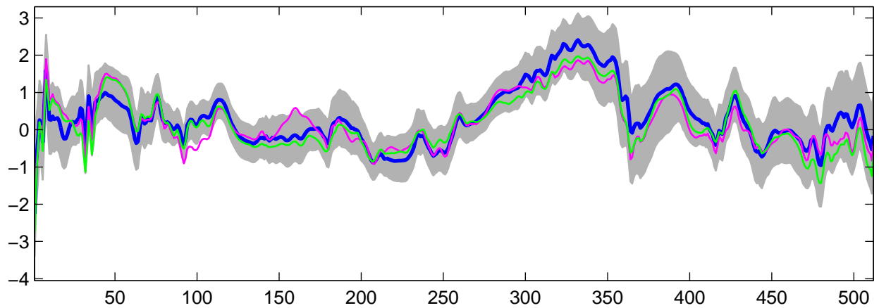
Estimated U_{14}(t) using R-WFMM: Normal data, run 8
