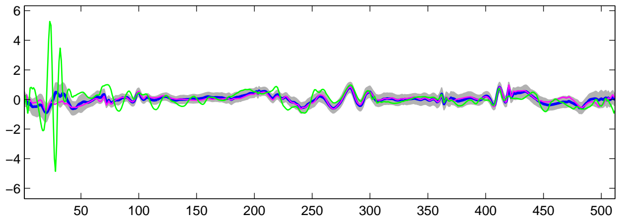
Estimated U_{14}(t) using R-WFMM: t_1 data, run 8
