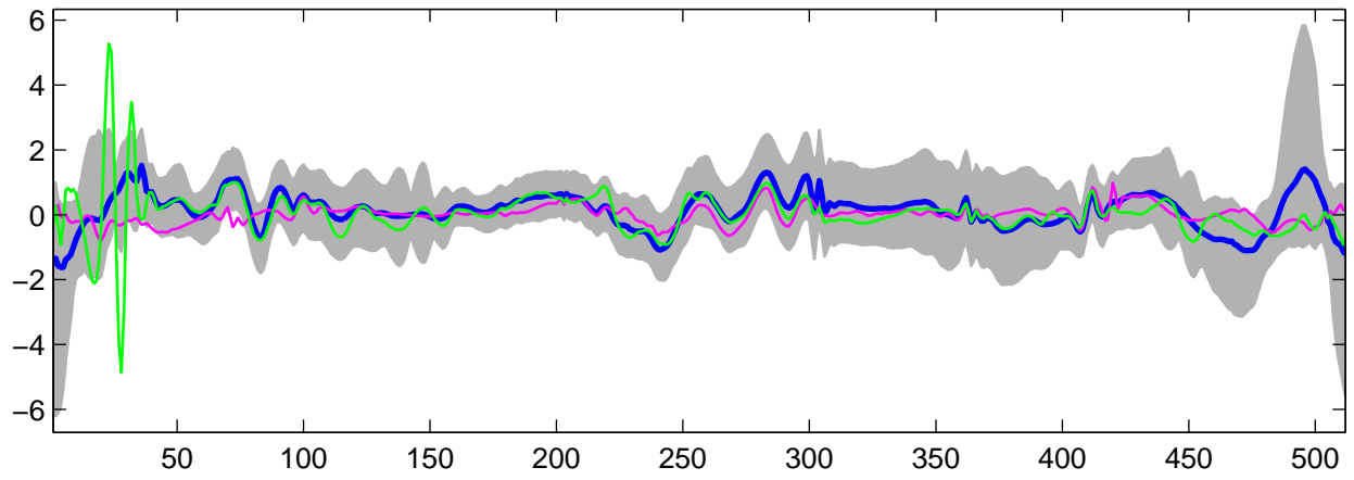
Estimated U_{14}(t) using G-WFMM: t_1 data, run 8
