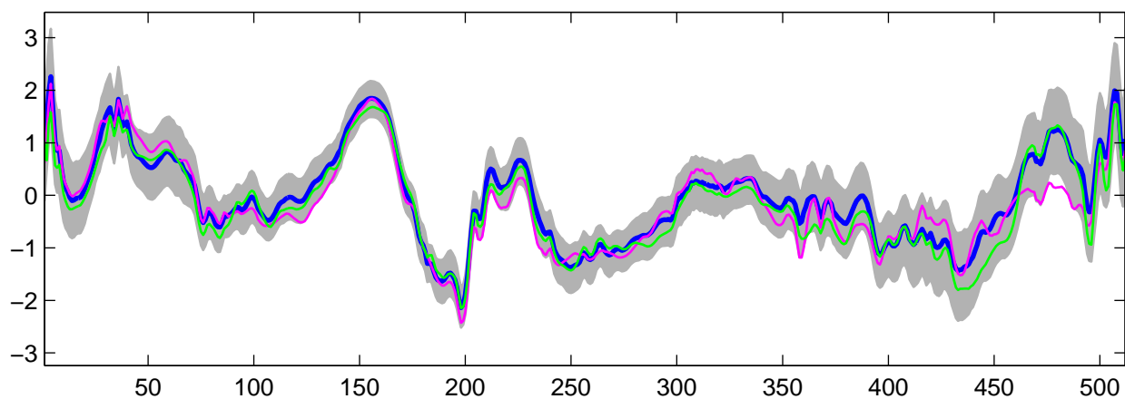
Estimated U_{14}(t) using R-WFMM: t_3 data, run 8
