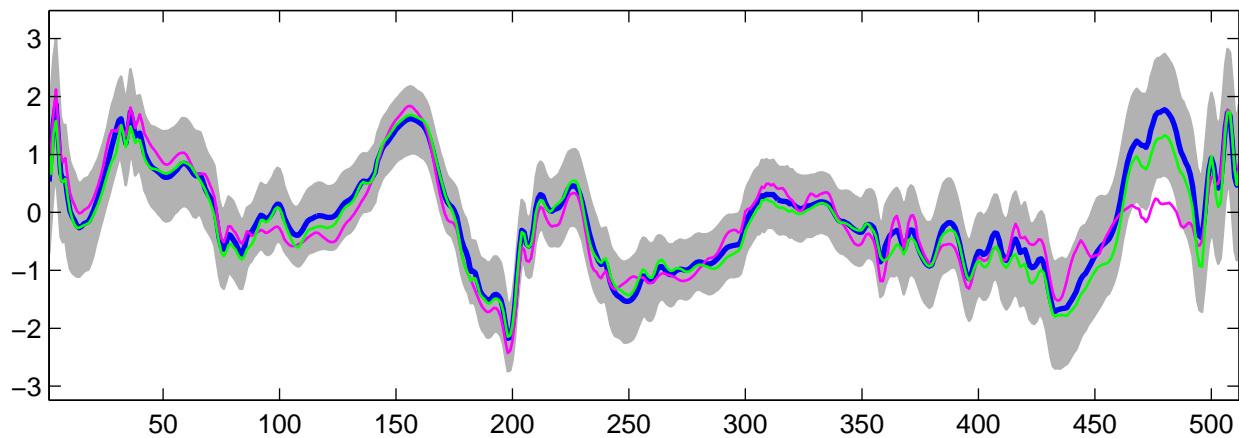
Estimated U_{14}(t) using G-WFMM: t_3 data, run 8
