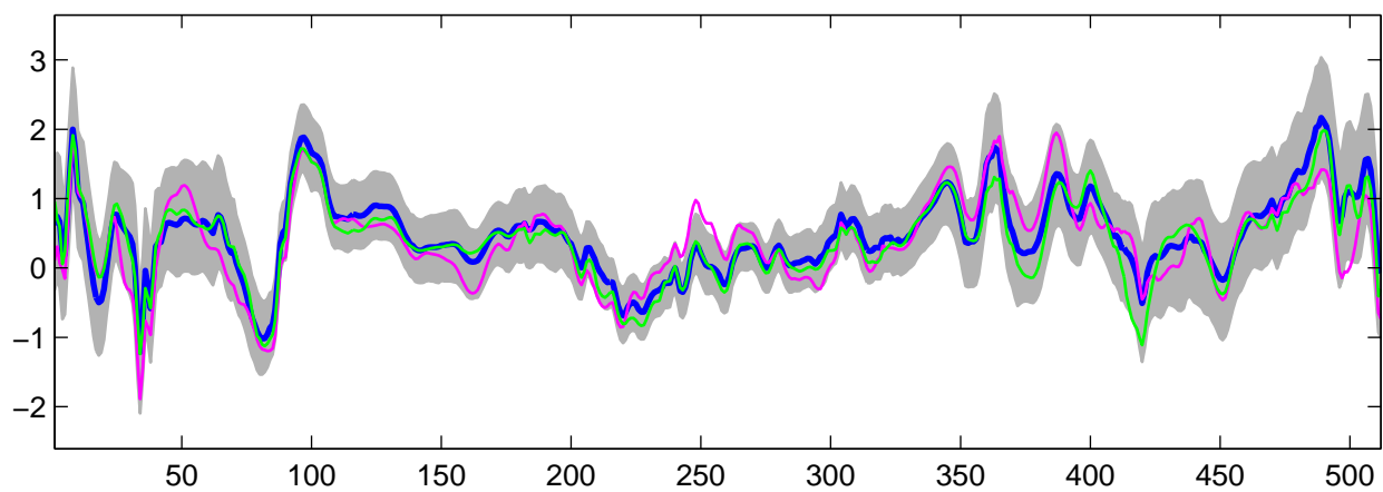
Estimated U_{15}(t) using R-WFMM: DE data, run 8
