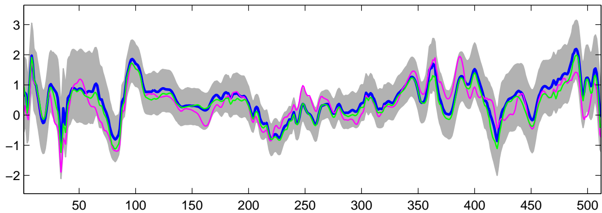
Estimated U_{15}(t) using G-WFMM: DE data, run 8
