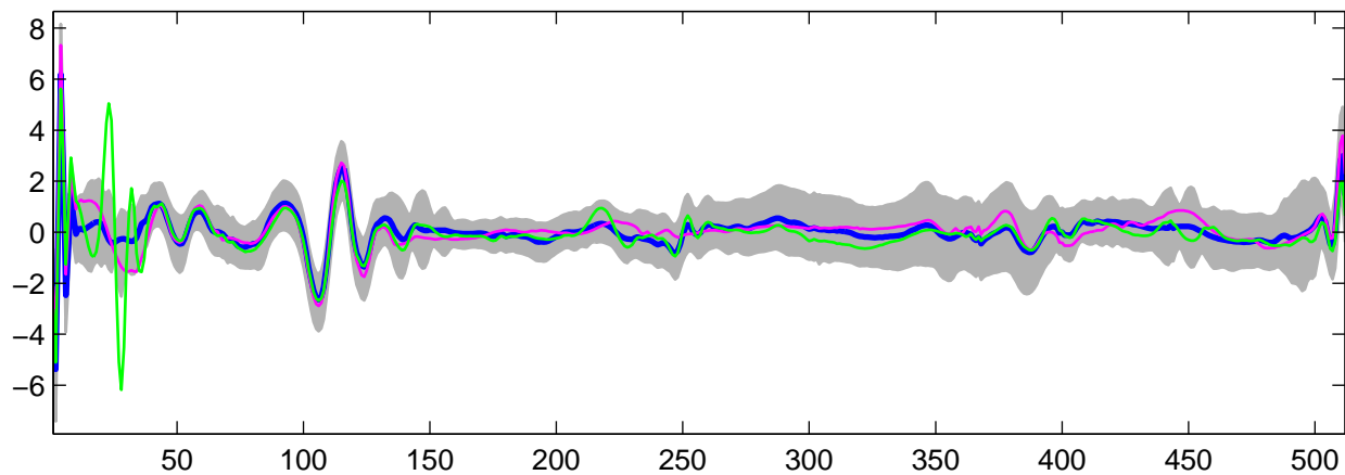
Estimated U_{15}(t) using G-WFMM: t_1 data, run 8
