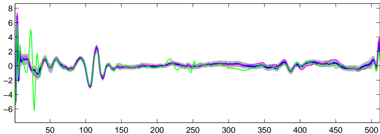
Estimated U_{15}(t) using R-WFMM: t_1 data, run 8
