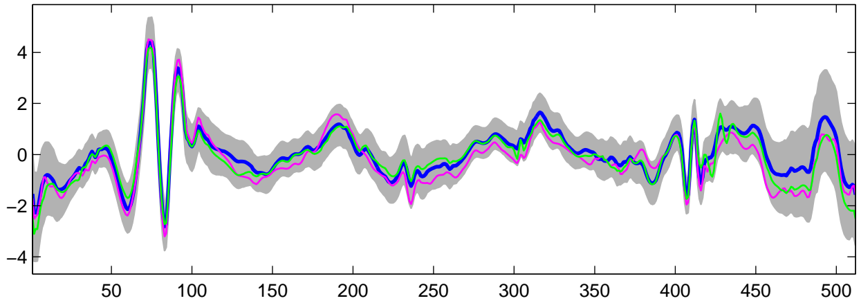
Estimated U_{15}(t) using G-WFMM: t_2 data, run 8
