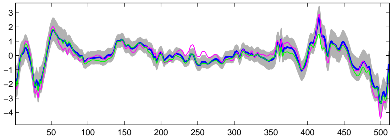
Estimated U_{16}(t) using R-WFMM: DE data, run 8
