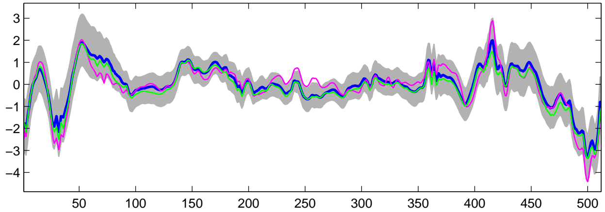
Estimated U_{16}(t) using G-WFMM: DE data, run 8
