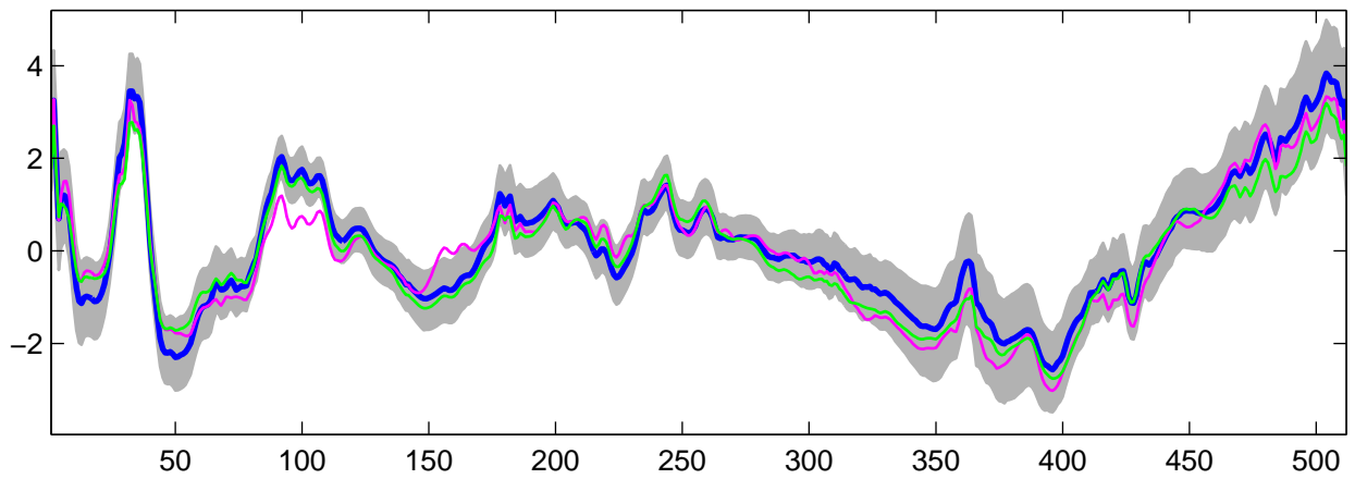
Estimated U_{16}(t) using R-WFMM: Normal data, run 8
