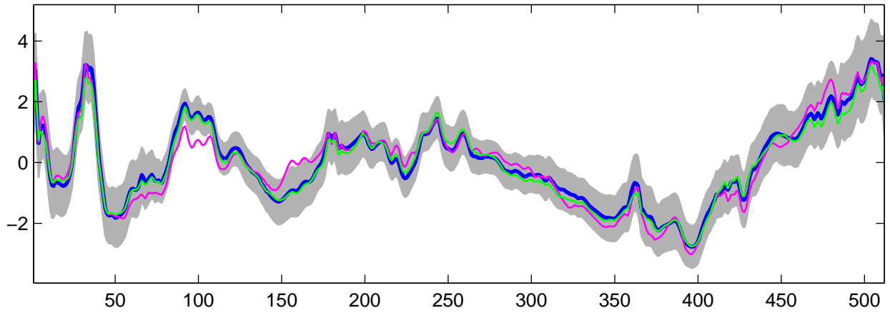
Estimated U_{16}(t) using G-WFMM: Normal data, run 8
