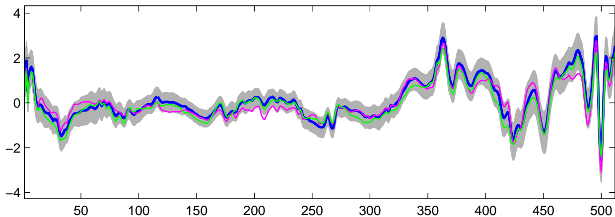
Estimated U_{16}(t) using R-WFMM: t_3 data, run 8
