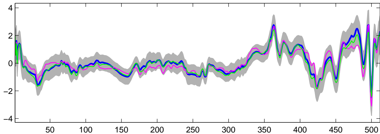
Estimated U_{16}(t) using G-WFMM: t_3 data, run 8
