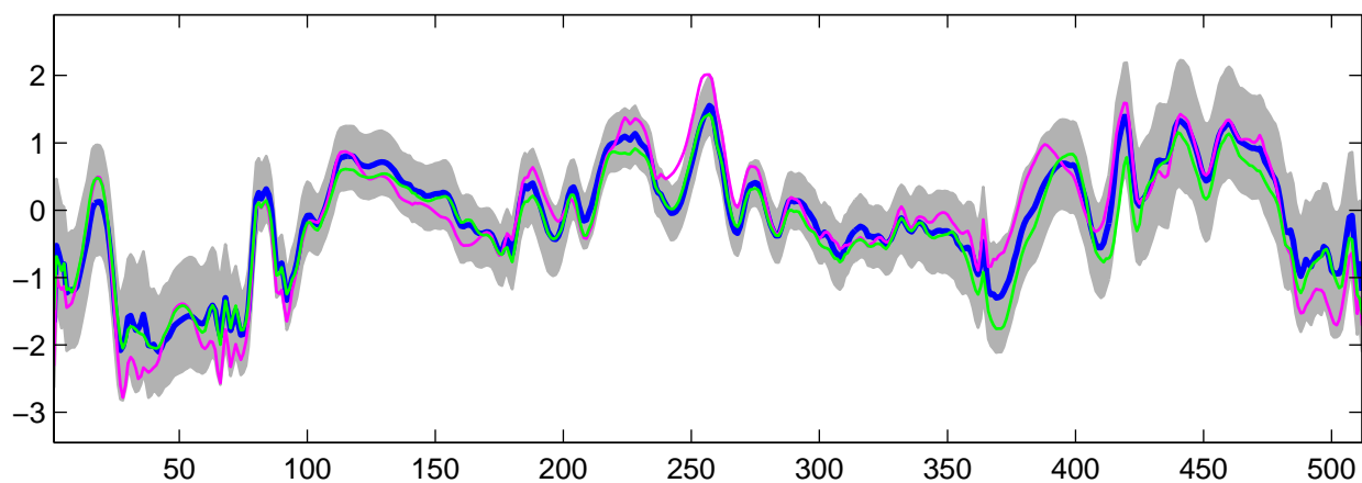
Estimated U_{17}(t) using R-WFMM: DE data, run 8
