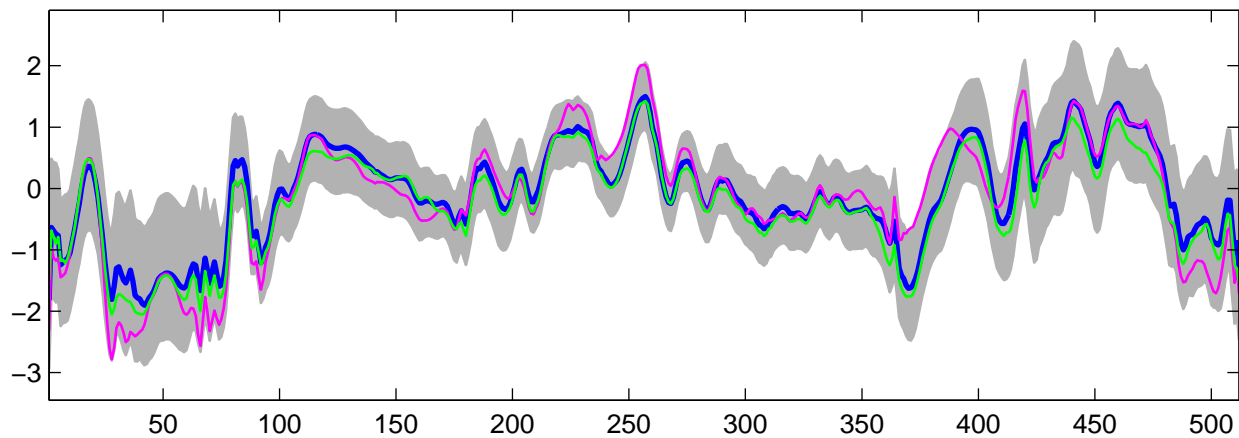
Estimated U_{17}(t) using G-WFMM: DE data, run 8
