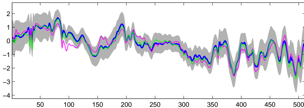
Estimated U_{17}(t) using G-WFMM: Normal data, run 8
