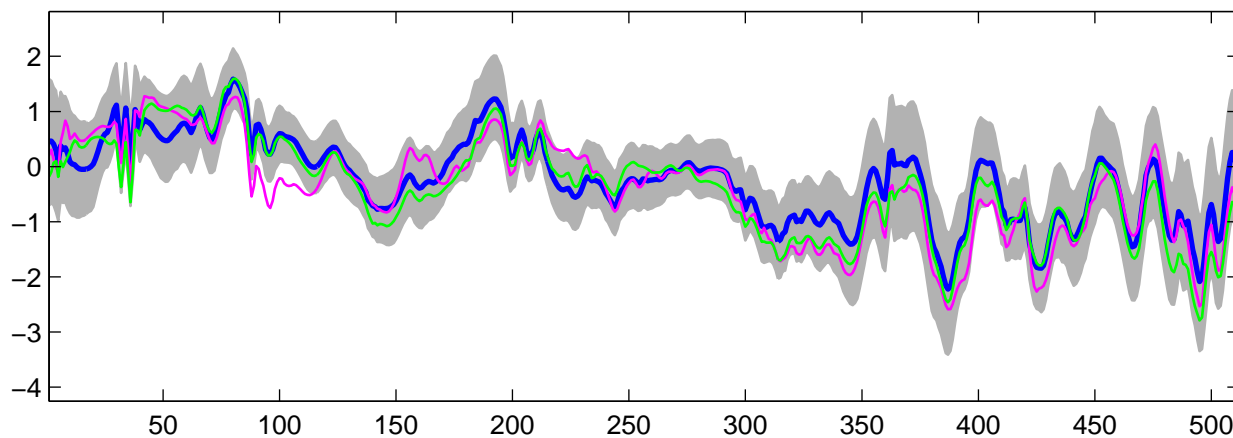
Estimated U_{17}(t) using R-WFMM: Normal data, run 8
