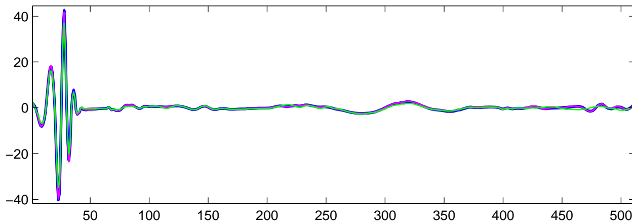
Estimated U_{17}(t) using R-WFMM: t_1 data, run 8
