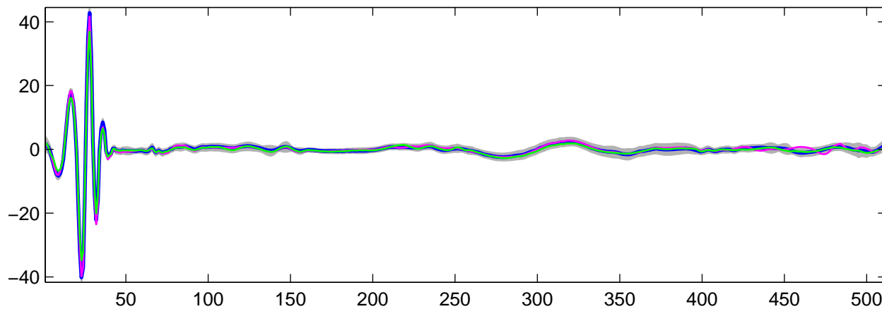
Estimated U_{17}(t) using G-WFMM: t_1 data, run 8
