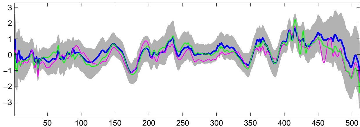
Estimated U_{17}(t) using G-WFMM: t_2 data, run 8
