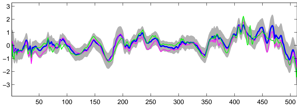
Estimated U_{17}(t) using R-WFMM: t_2 data, run 8
