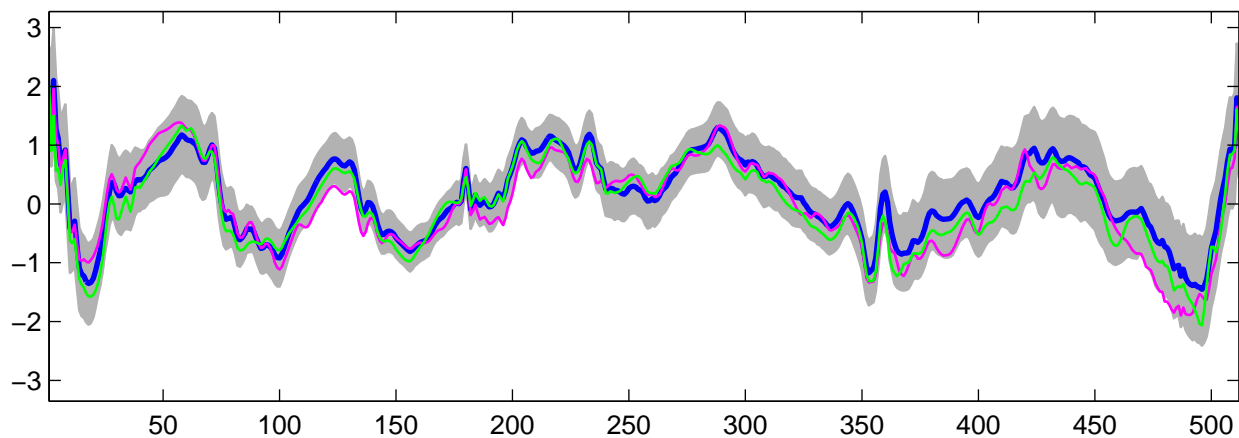
Estimated U_{17}(t) using R-WFMM: t_3 data, run 8
