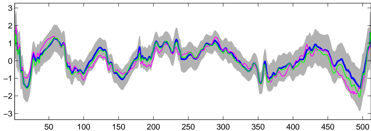
Estimated U_{17}(t) using G-WFMM: t_3 data, run 8
