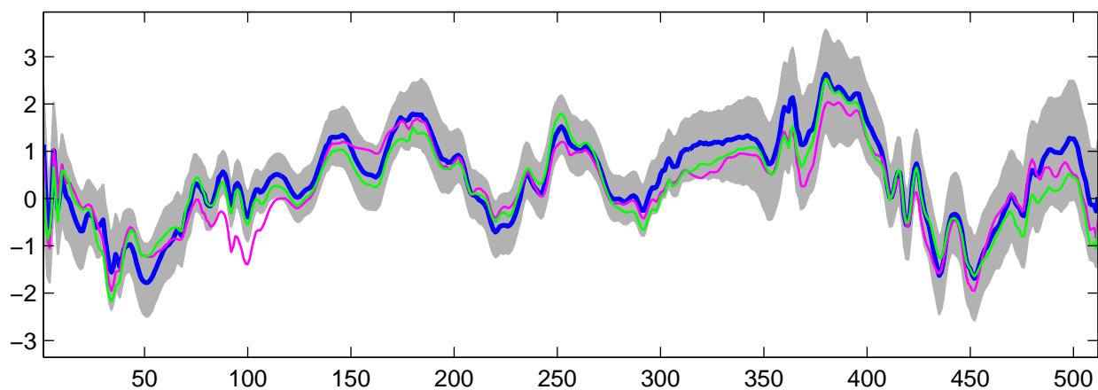
Estimated U_{18}(t) using R-WFMM: Normal data, run 8
