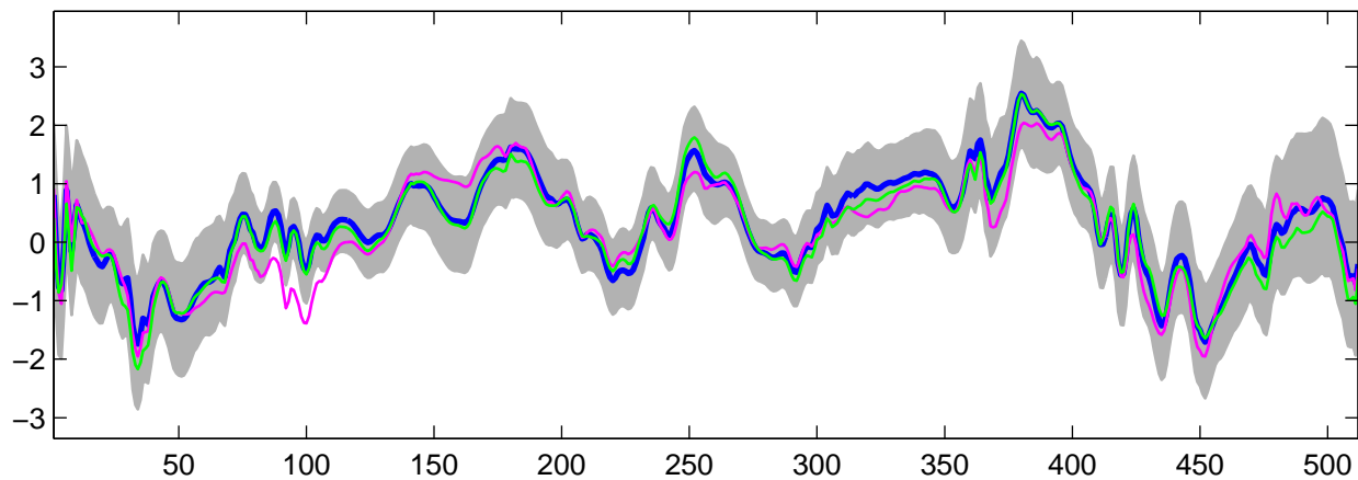
Estimated U_{18}(t) using G-WFMM: Normal data, run 8
