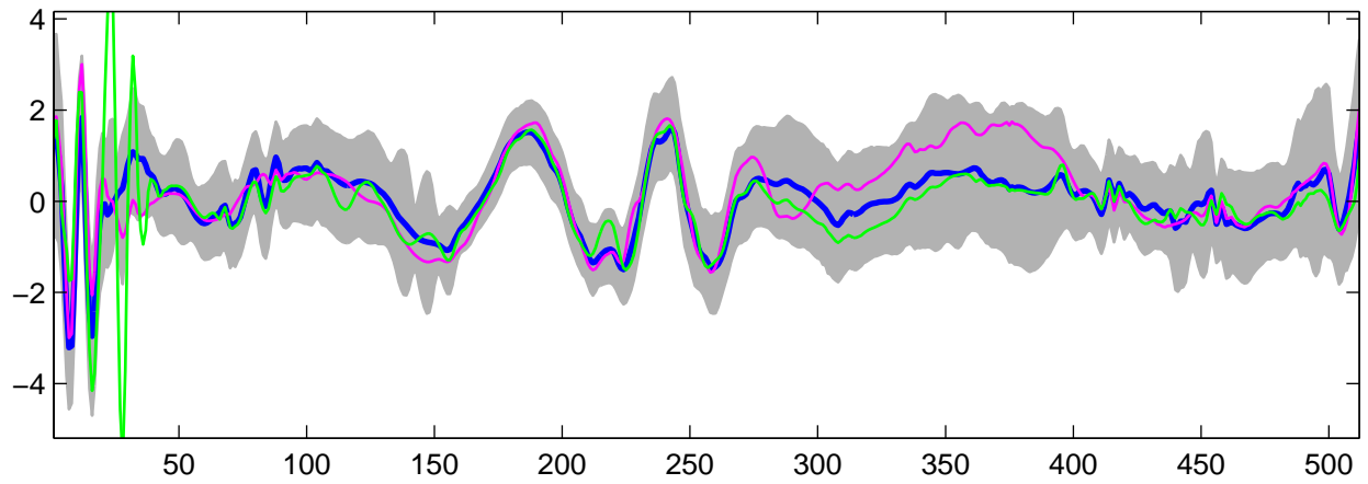
Estimated U_{18}(t) using G-WFMM: t_1 data, run 8
