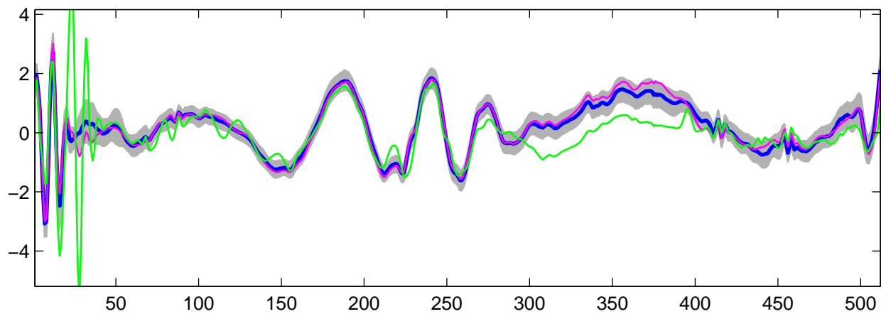
Estimated U_{18}(t) using R-WFMM: t_1 data, run 8
