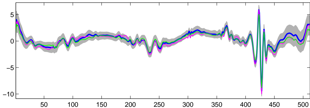
Estimated U_{18}(t) using G-WFMM: t_2 data, run 8
