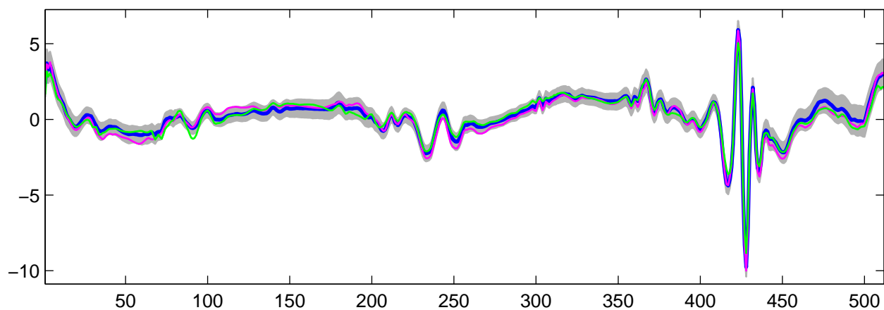
Estimated U_{18}(t) using R-WFMM: t_2 data, run 8
