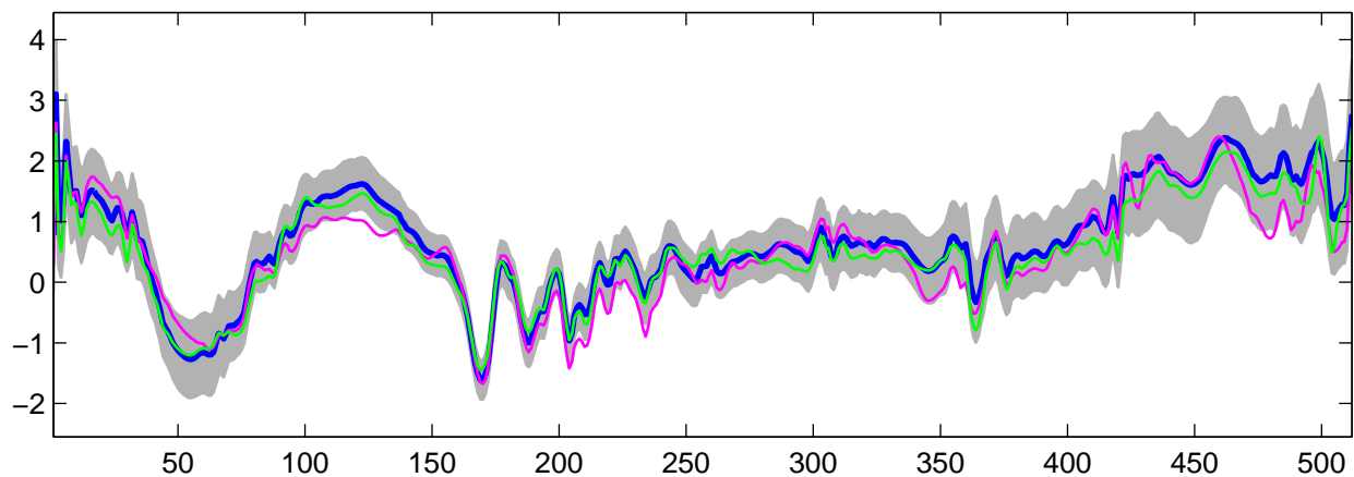
Estimated U_{18}(t) using R-WFMM: t_3 data, run 8
