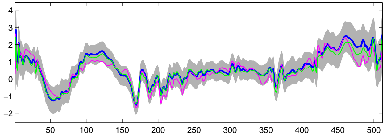
Estimated U_{18}(t) using G-WFMM: t_3 data, run 8
