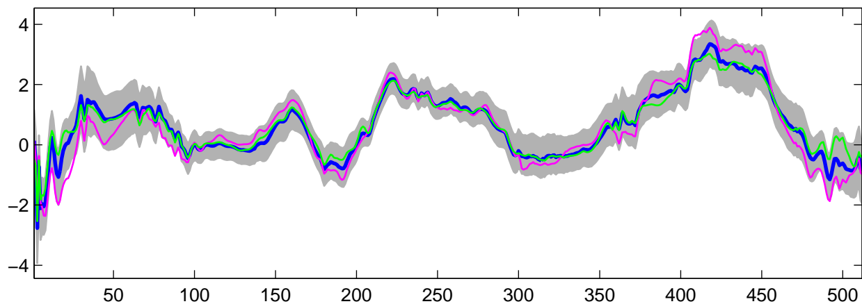
Estimated U_{19}(t) using R-WFMM: DE data, run 8
