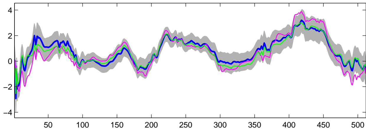
Estimated U_{19}(t) using G-WFMM: DE data, run 8
