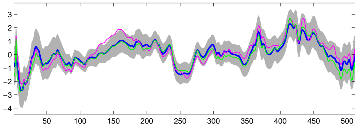
Estimated U_{19}(t) using G-WFMM: Normal data, run 8
