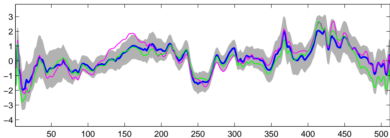
Estimated U_{19}(t) using R-WFMM: Normal data, run 8
