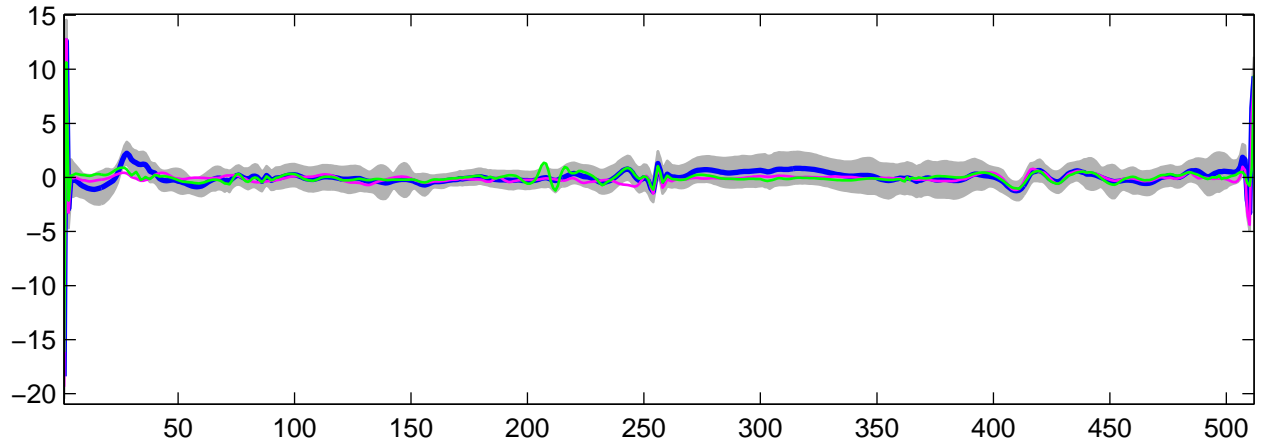
Estimated U_{19}(t) using G-WFMM: t_1 data, run 8
