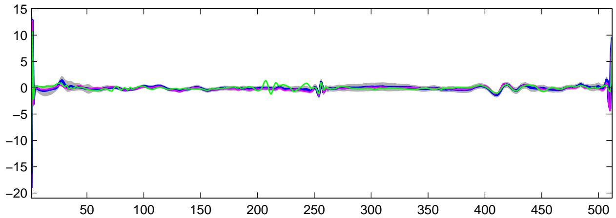
Estimated U_{19}(t) using R-WFMM: t_1 data, run 8
