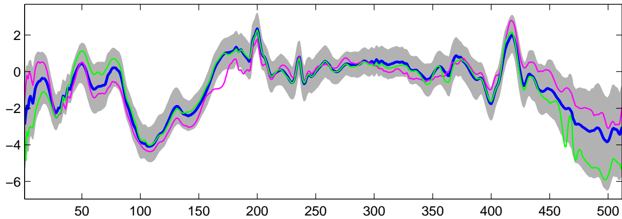
Estimated U_{19}(t) using G-WFMM: t_2 data, run 8
