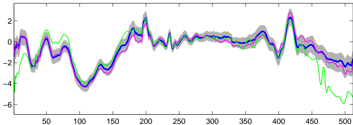
Estimated U_{19}(t) using R-WFMM: t_2 data, run 8
