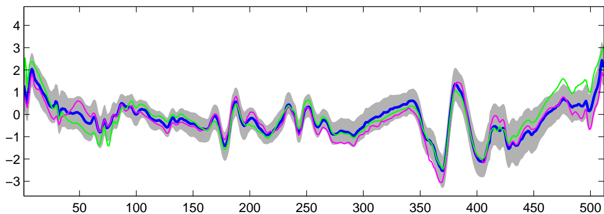
Estimated U_{19}(t) using R-WFMM: t_3 data, run 8
