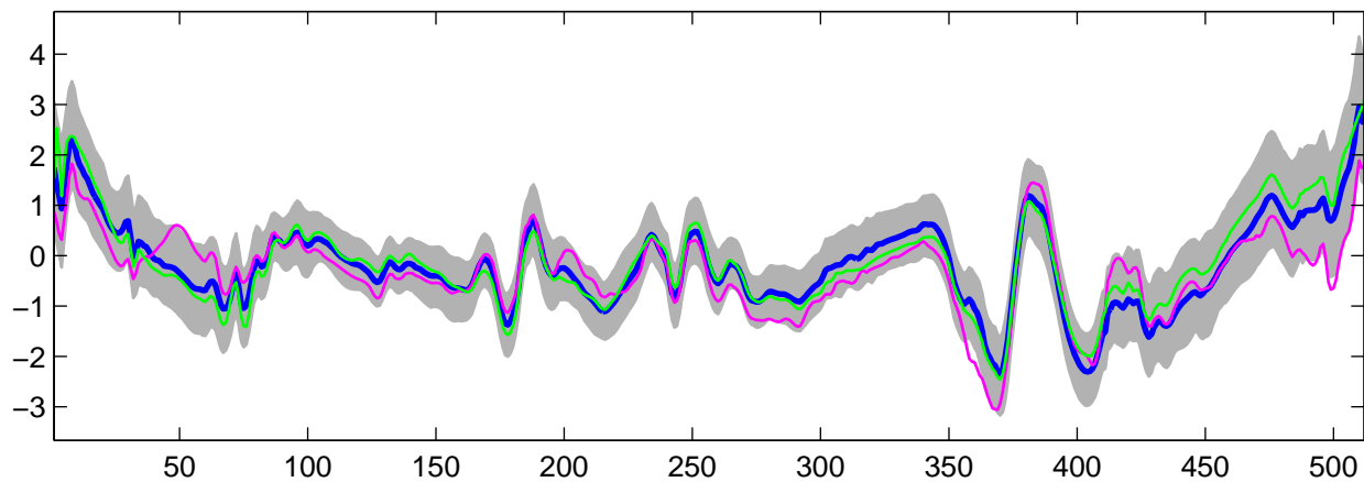
Estimated U_{19}(t) using G-WFMM: t_3 data, run 8
