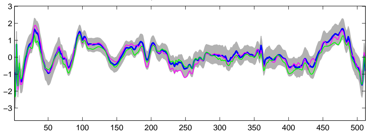
Estimated U_1(t) using R-WFMM: DE data, run 8
