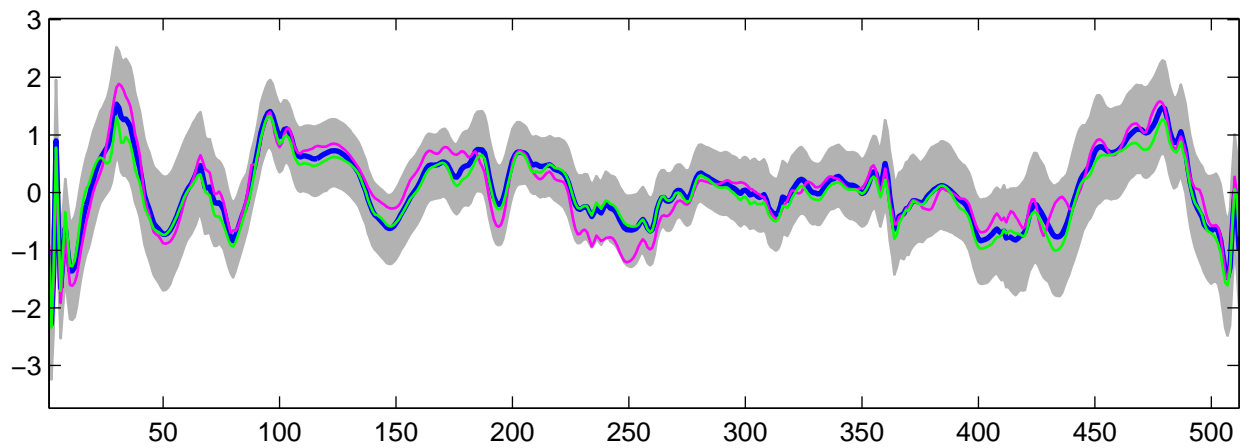
Estimated U_1(t) using G-WFMM: DE data, run 8
