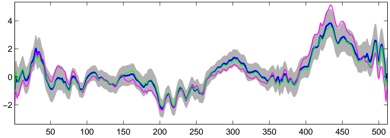
Estimated U_1(t) using G-WFMM: Normal data, run 8
