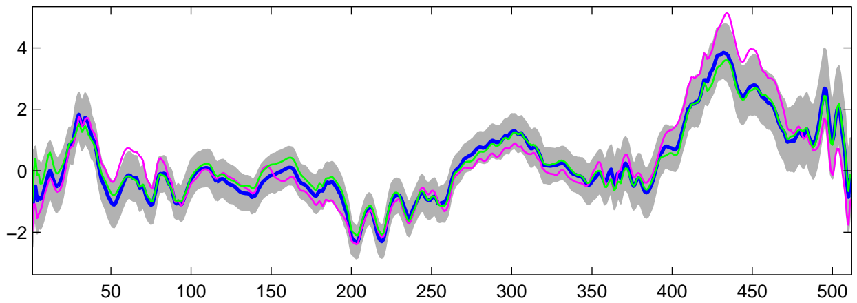
Estimated U_1(t) using R-WFMM: Normal data, run 8
