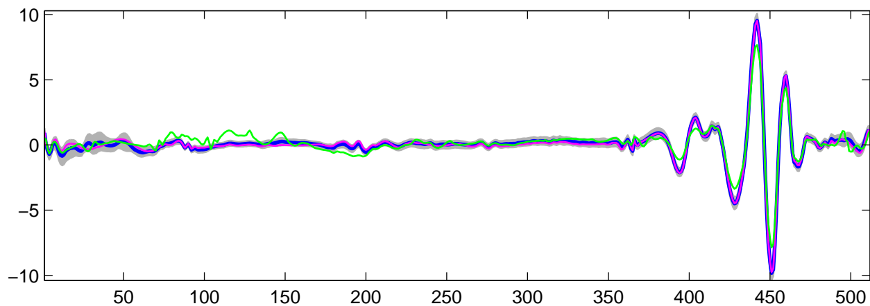
Estimated U_1(t) using R-WFMM: t_1 data, run 8
