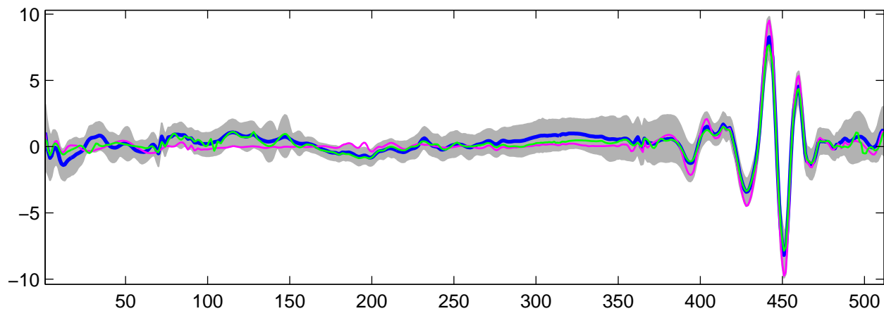
Estimated U_1(t) using G-WFMM: t_1 data, run 8
