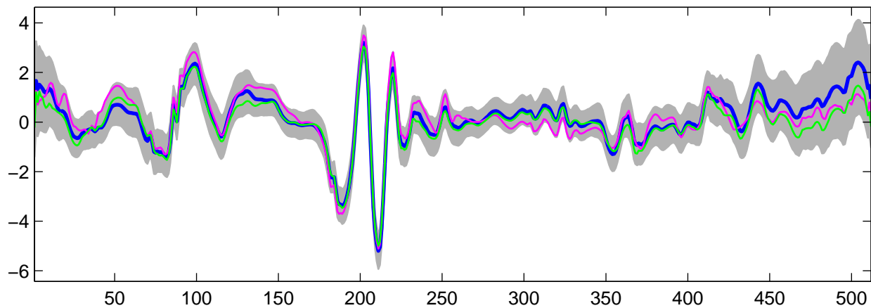
Estimated U_1(t) using G-WFMM: t_2 data, run 8
