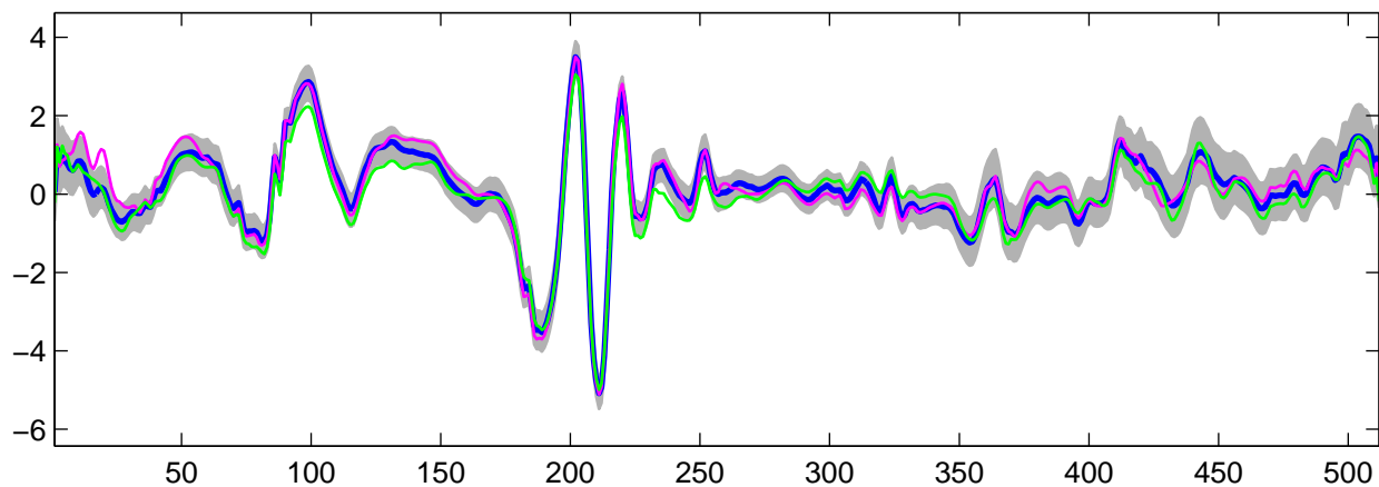
Estimated U_1(t) using R-WFMM: t_2 data, run 8
