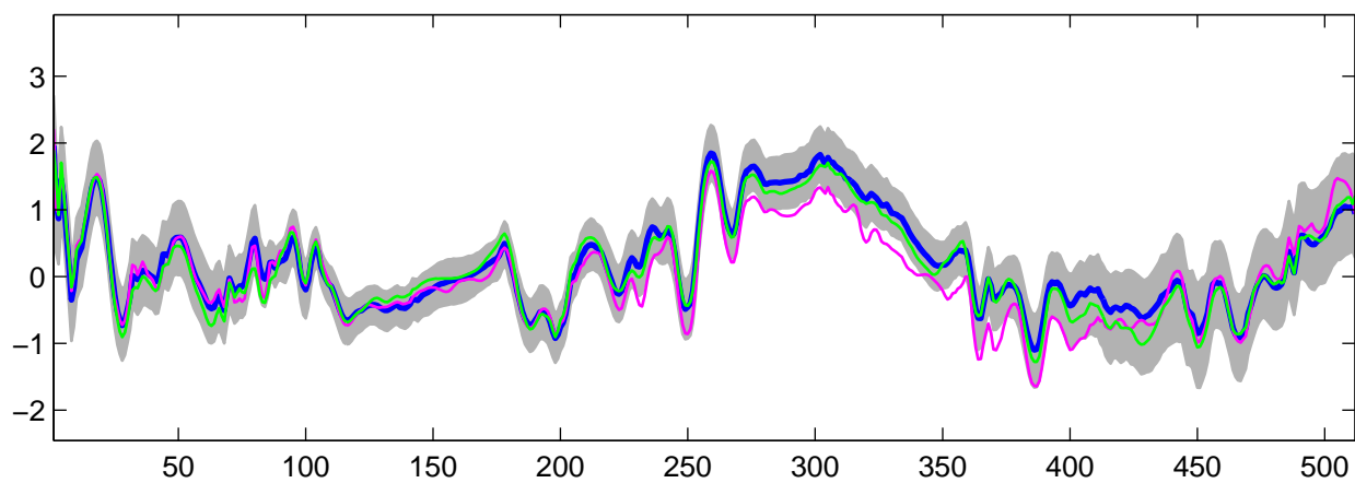
Estimated U_1(t) using R-WFMM: t_3 data, run 8
