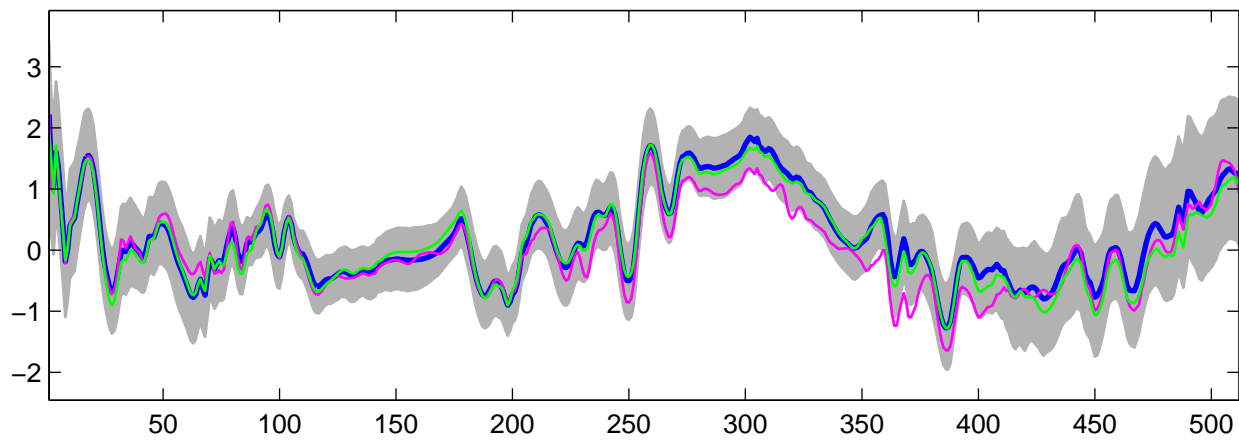
Estimated U_1(t) using G-WFMM: t_3 data, run 8
