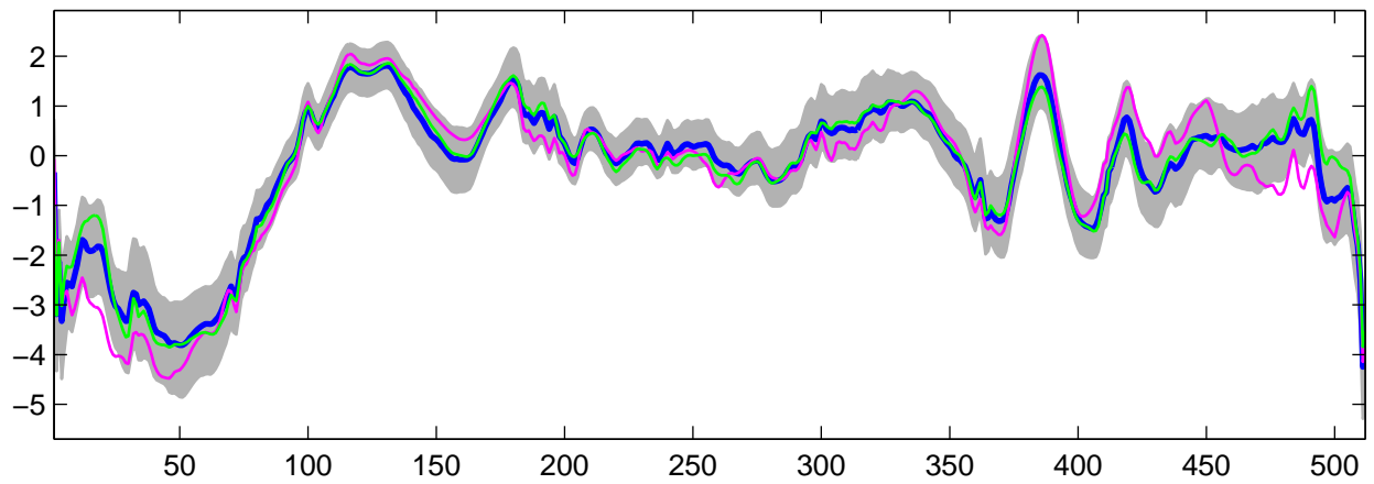
Estimated U_{20}(t) using R-WFMM: DE data, run 8
