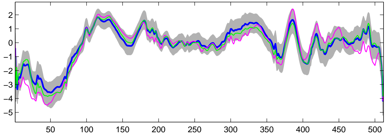
Estimated U_{20}(t) using G-WFMM: DE data, run 8
