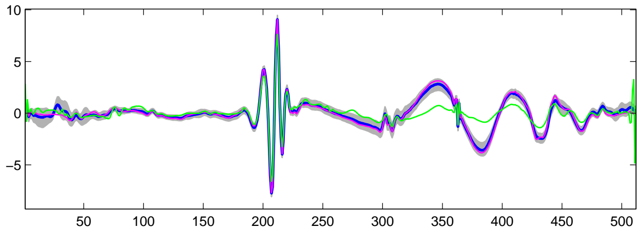
Estimated U_{20}(t) using R-WFMM: t_1 data, run 8
