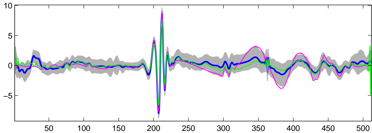
Estimated U_{20}(t) using G-WFMM: t_1 data, run 8
