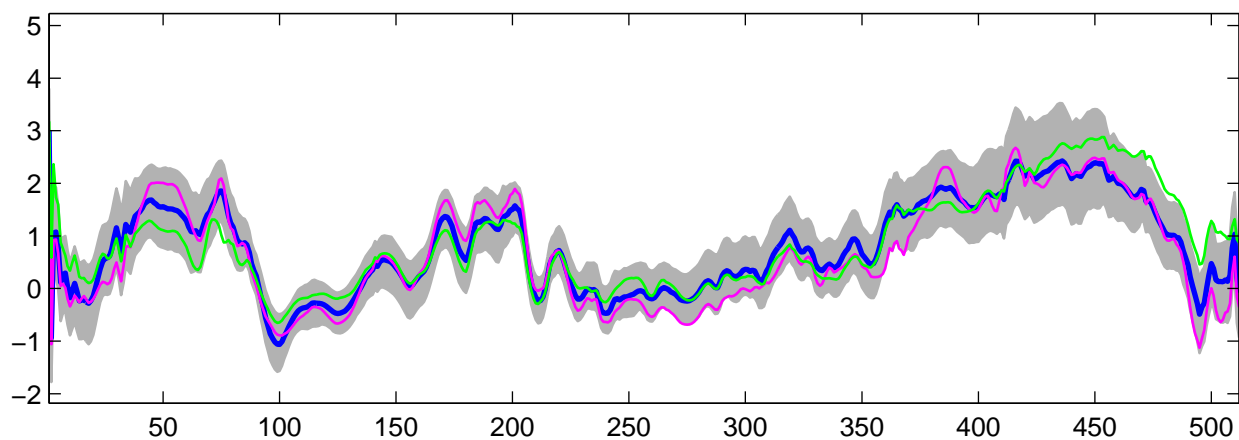
Estimated U_{20}(t) using R-WFMM: t_3 data, run 8
