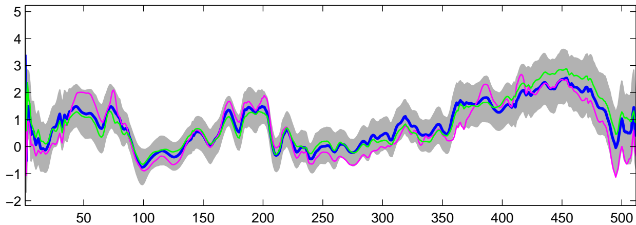
Estimated U_{20}(t) using G-WFMM: t_3 data, run 8
