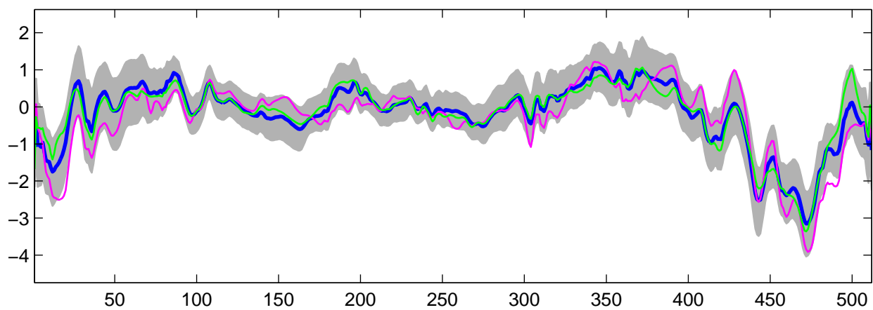
Estimated U_{21}(t) using R-WFMM: DE data, run 8
