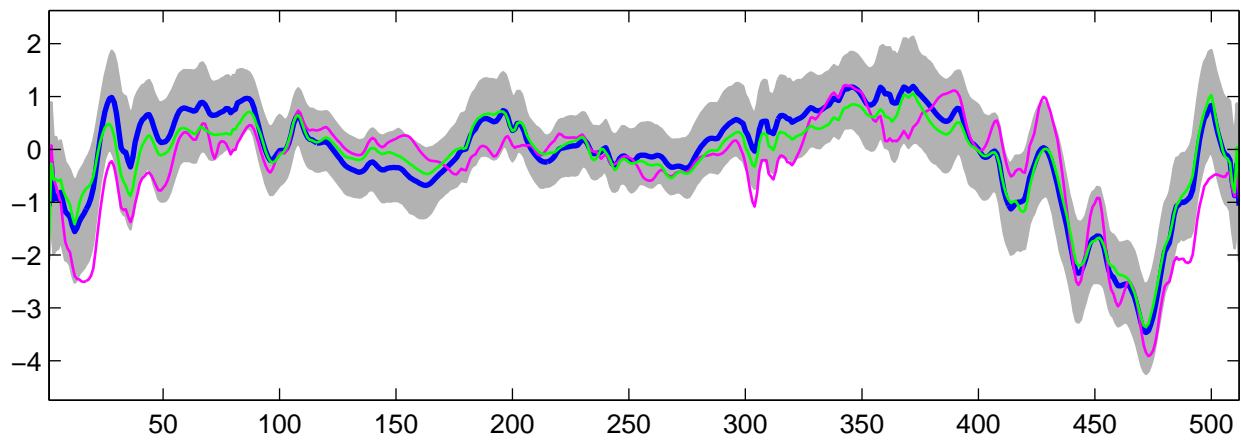
Estimated U_{21}(t) using G-WFMM: DE data, run 8
