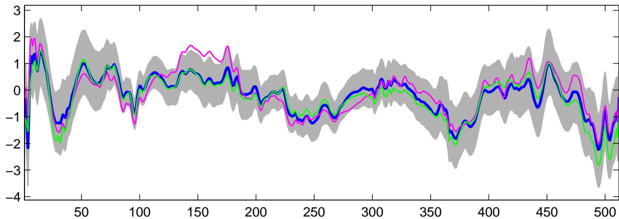
Estimated U_{21}(t) using G-WFMM: Normal data, run 8
