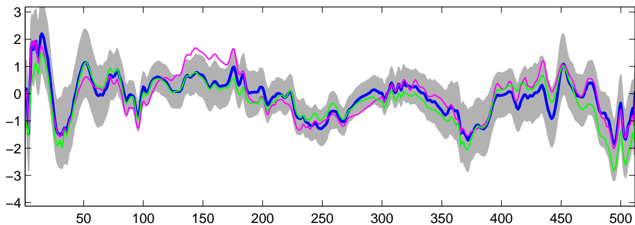
Estimated U_{21}(t) using R-WFMM: Normal data, run 8
