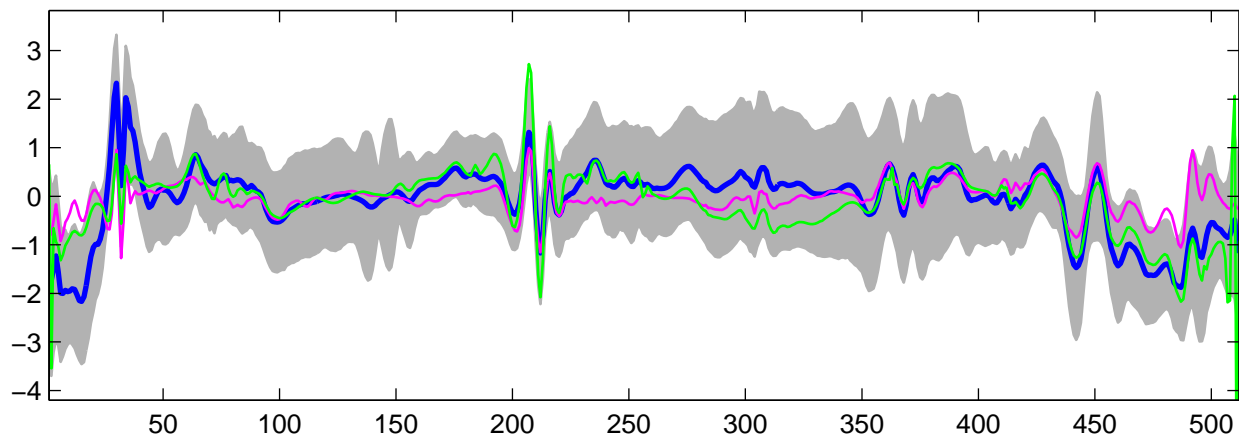
Estimated U_{21}(t) using G-WFMM: t_1 data, run 8
