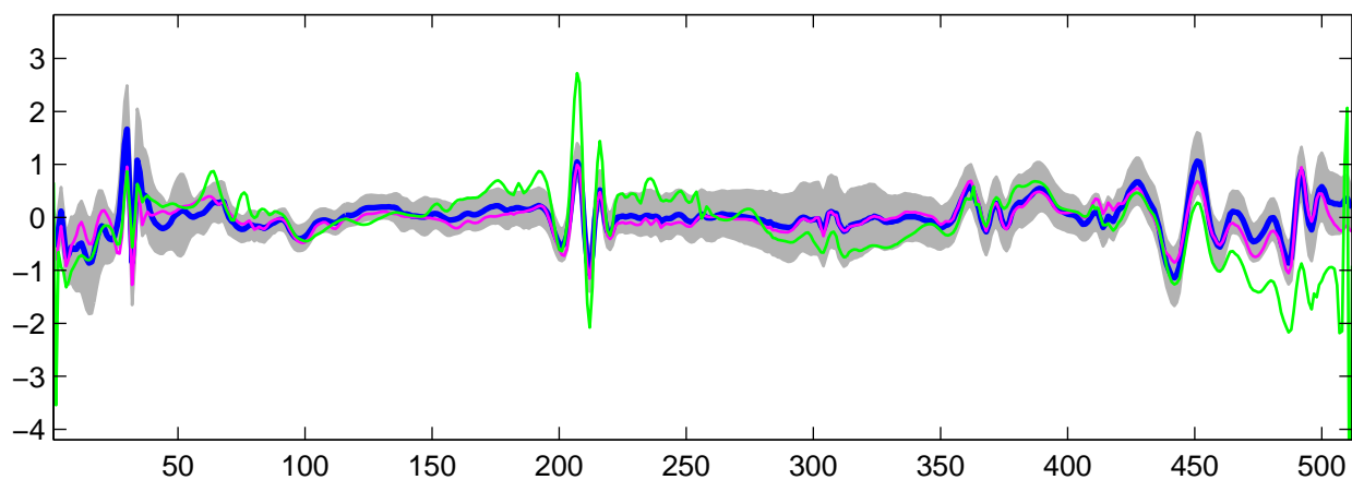
Estimated U_{21}(t) using R-WFMM: t_1 data, run 8
