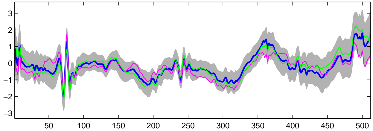
Estimated U_{21}(t) using G-WFMM: t_3 data, run 8
