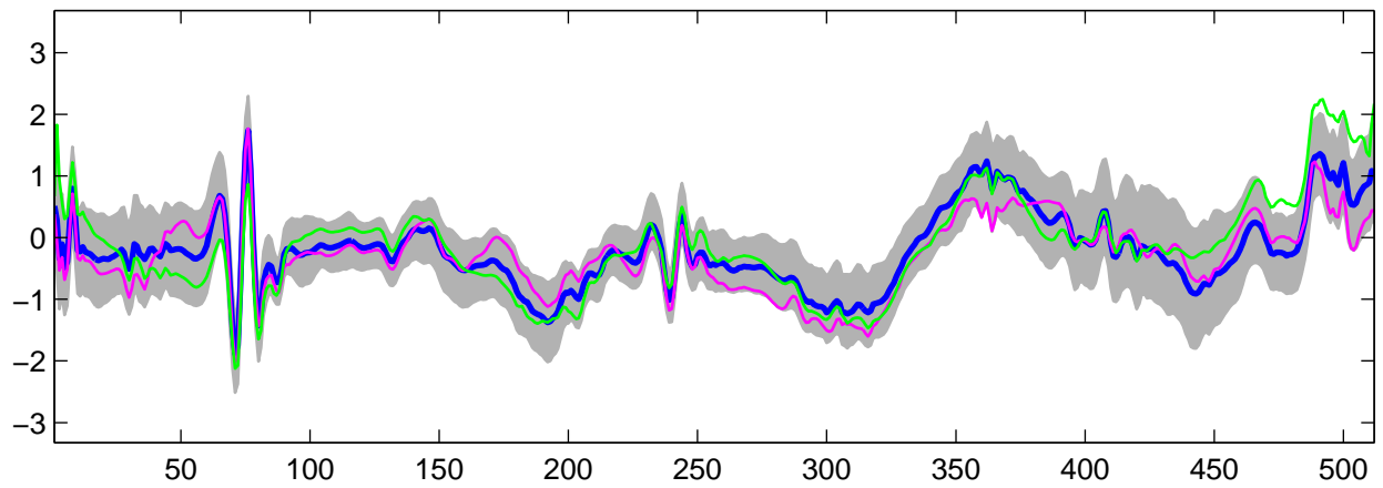
Estimated U_{21}(t) using R-WFMM: t_3 data, run 8
