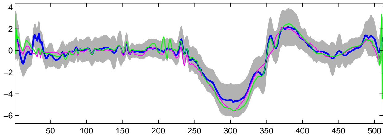
Estimated U_{22}(t) using G-WFMM: t_1 data, run 8
