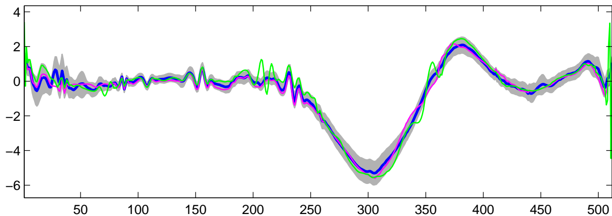
Estimated U_{22}(t) using R-WFMM: t_1 data, run 8
