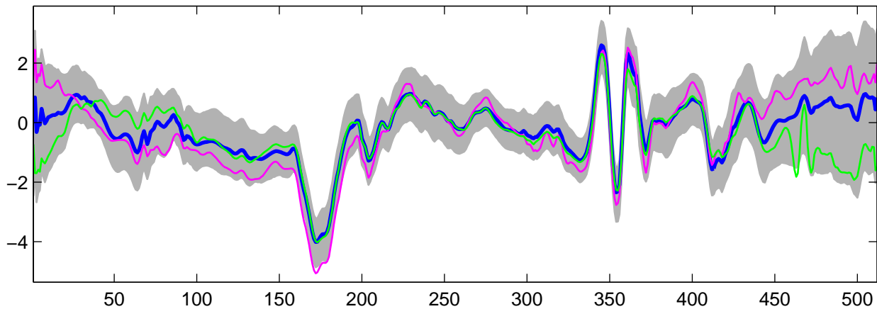
Estimated U_{22}(t) using G-WFMM: t_2 data, run 8
