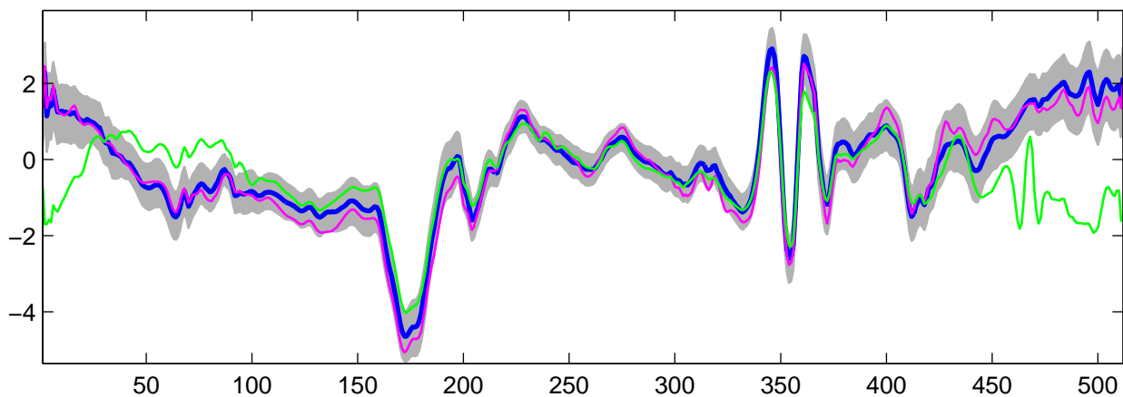
Estimated U_{22}(t) using R-WFMM: t_2 data, run 8
